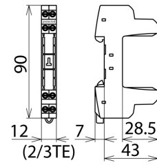
Dimension drawing BSP BAS 4
